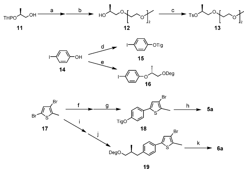
Scheme 3. Synthesis of compounds 5a and 6a . Reagents and conditions: a) TsODeg, NaH, dry THF; b) PPTS, EtOH, 81% in two steps; c) TsCl, aq. NaOH, THF, 60%; d) TsOTig, K_2CO_3 , DMF, 99%; e) 13 , K_2CO_3 , DMF, quantitative; f) n BuLi, dry THF, and then (BuO)_3B ; g) 15 , THF, aq. Na_2CO_3 , Pd(PPh_3)_4 , 85% in two steps; h) n BuLi, dry THF, and then perfluorocyclopentene, 25%; i) n BuLi, dry THF, and then (BuO)_3B ; j) 16 , THF, aq. Na_2CO_3 , Pd(PPh_3)_4 , 76% in two steps; k) n BuLi, dry THF, and then perfluorocyclopentene, 21%.
