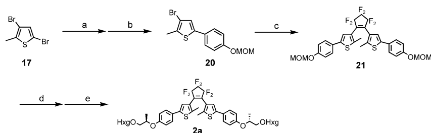
Scheme 4. Synthesis of compound 2a by Mitsunobu Reaction. Reagents and conditions: a) n BuLi, dry THF, and then (BuO)_3B ; b) 1-iodo-4-methoxymethoxybenzene, THF, aq. Na_2CO_3 , Pd(PPh_3)_4 , 88% in two steps; c) n BuLi, dry THF, and then perfluorocyclopentene, 40%; d) conc. HCl, THF; e) DEAD, PPh_3 , then ( S )-HOCHMeCH 2 OHxg, THF, 16% in two steps.
