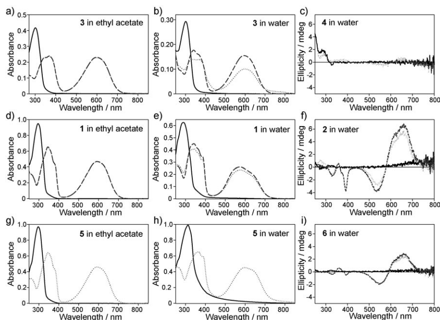
Figure 1. Absorption and CD spectra of diarylethenes along with photochromism: Absorption spectra of compounds 1 , 3 , and 5 in ethyl acetate (left column), in water (center column), and the corresponding CD spectra of compounds 2 , 4 , and 6 in water (right column). (a)–(c): 3 and 4 ; (d)–(f): 1 and 2 ; (g)–(i): 5 and 6 . Black solid line: open-ring isomer; dark gray dashed line: closed-ring isomer; pale gray dotted line: sample in the photostationary state under irradiation with 313 nm light.
