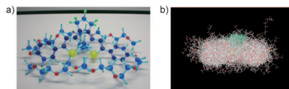
Figure 5. a) Molecular model of compound 1b . When the length of PEG side chain is n=6 (Hxg), the diarylethene core would be surrounded by the amphiphilic side chains moderately. b) The result of the molecular mechanics calculation. The superimposed structures of the most stable 100 conformers are shown. Elements are colored as follows: C grey, H white, O red, F green.
