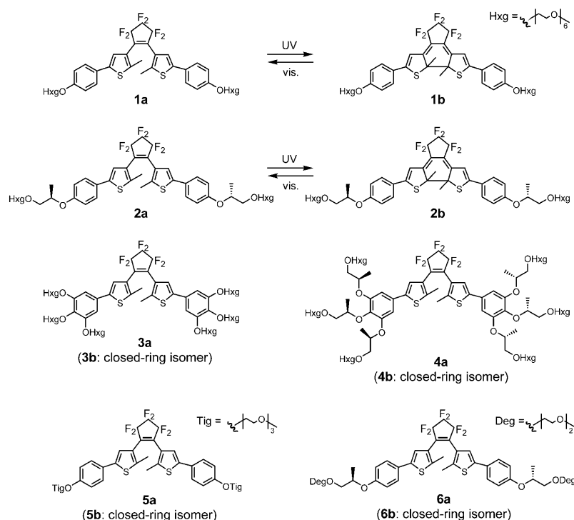
Scheme 1. Photochromism of diarylethenes having PEG side chains.
