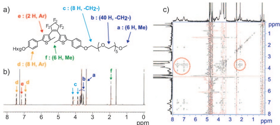
Figure 4. a) The molecular structure of compound 1 . b) ^1\text{H} NMR spectrum of the open-ring isomer 1a in \text{CDCl}_3 at room temperature. c) NOESY spectrum of the sample in the photostationary state under irradiation with 313 nm light (91 % closed-ring isomer) in \text{D}_2\text{O} at 50 °C (400 MHz; mixing time, 0.3 sec). NOEs between protons of PEG side chains (a–c) and protons of diarylethene (d–f) were detected (red dashed circles).
