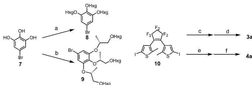
Scheme 2. Synthesis of compounds 3a and 4a . Reagents and conditions: a) TsOHxg, K_2CO_3 , DMF, 86%; b) ( S )-TsOCHMeCH 2 OHxg, K_2CO_3 , DMF, 42%; c) n BuLi, dry THF, and then (BuO)_3B ; d) 8 , THF, aq. Na_2CO_3 , Pd(PPh_3)_4 , 9% in two steps; e) n BuLi, dry THF, and then 2-isopropoxy-4,4,5,5-tetramethyl-1,3,2-dioxaborolane; f) 9 , THF, aq. Na_2CO_3 , Pd(PPh_3)_4 , 12% in two steps.
