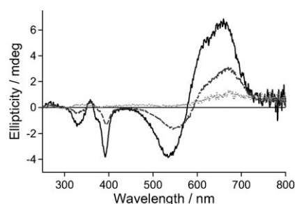
Figure 2. CD spectra of compound 2 in water (black solid line), in MeOH/H 2 O=25:75 (dark gray dashed line), and in MeOH/H 2 O=50:50 (pale gray dotted line).
