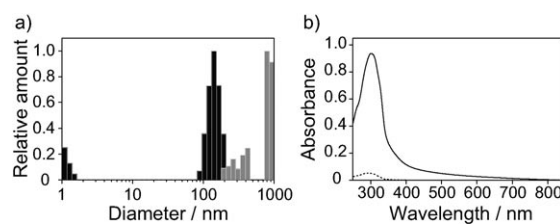
Figure 3. a) Size distribution of the open-ring isomer 5a in water before filtration (gray bar) and after filtration (black bar). b) The concentration change of an aqueous solution of compound 5a before (solid line) and after (dashed line) filtration with a 0.2 \mu m membrane filter.
